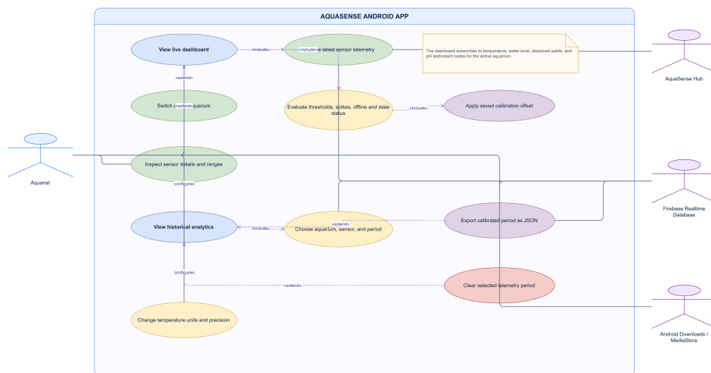
Figure 2: Use case diagram for monitoring analytics.
