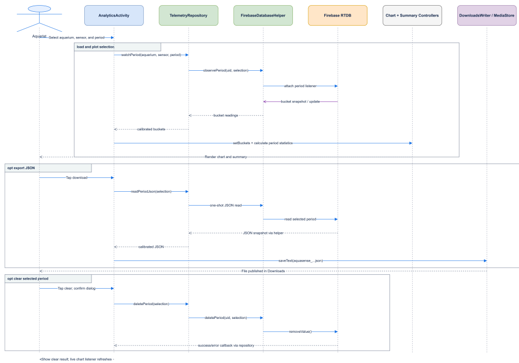
Figure 5: Sequence diagram for analytics.
