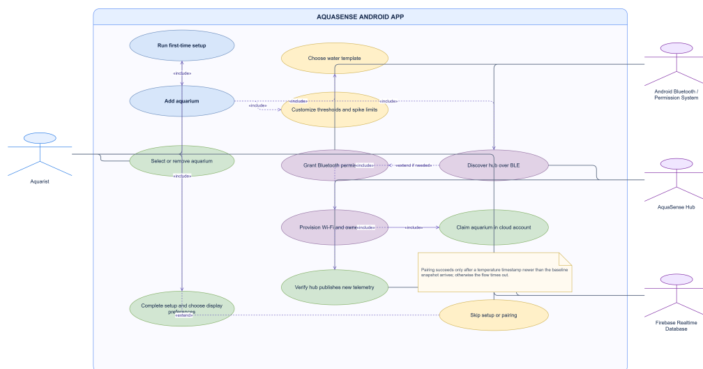
Figure 4: Use case diagram for setup pairing.
