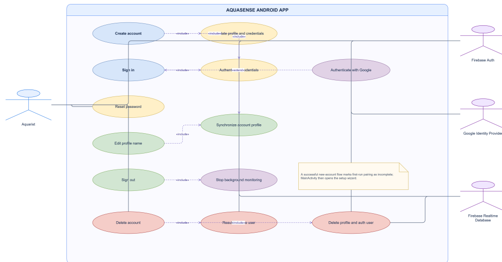
Figure 1: Use case diagram for account access.
