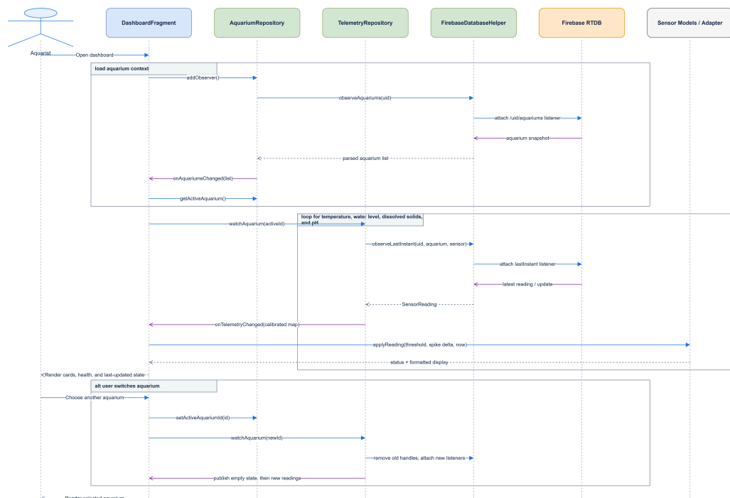
Figure 8: Sequence diagram for live dashboard.
