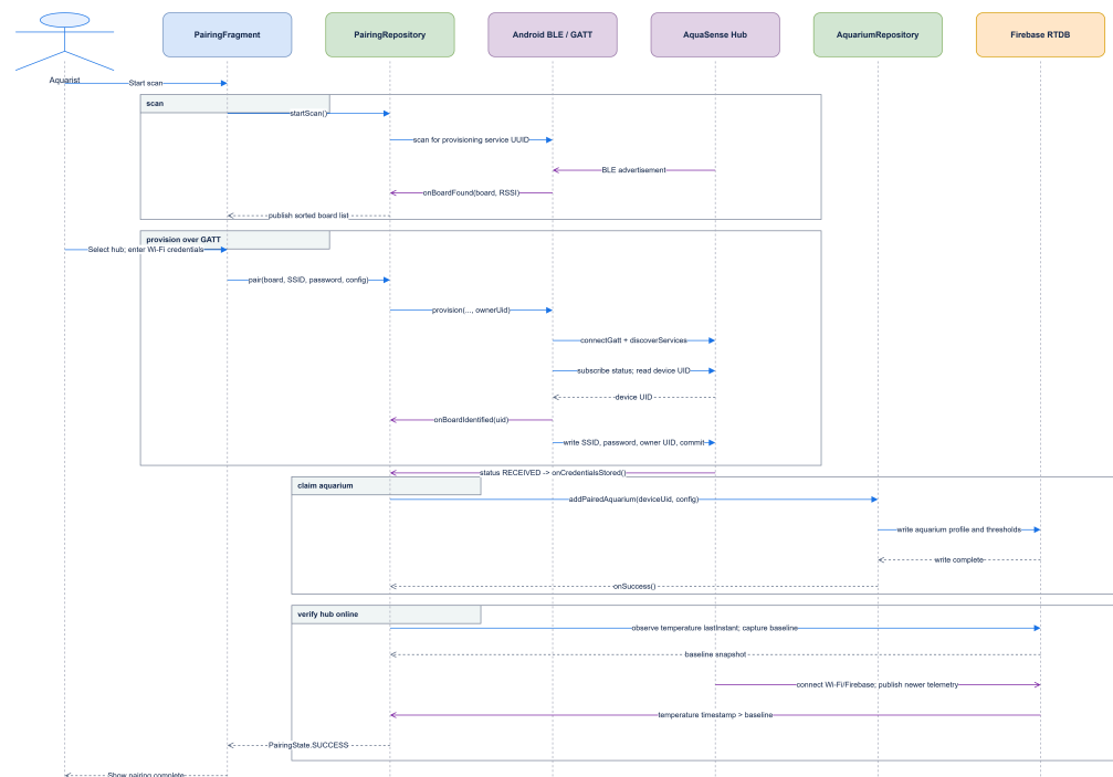
Figure 6: Sequence diagram for aquarium pairing.
